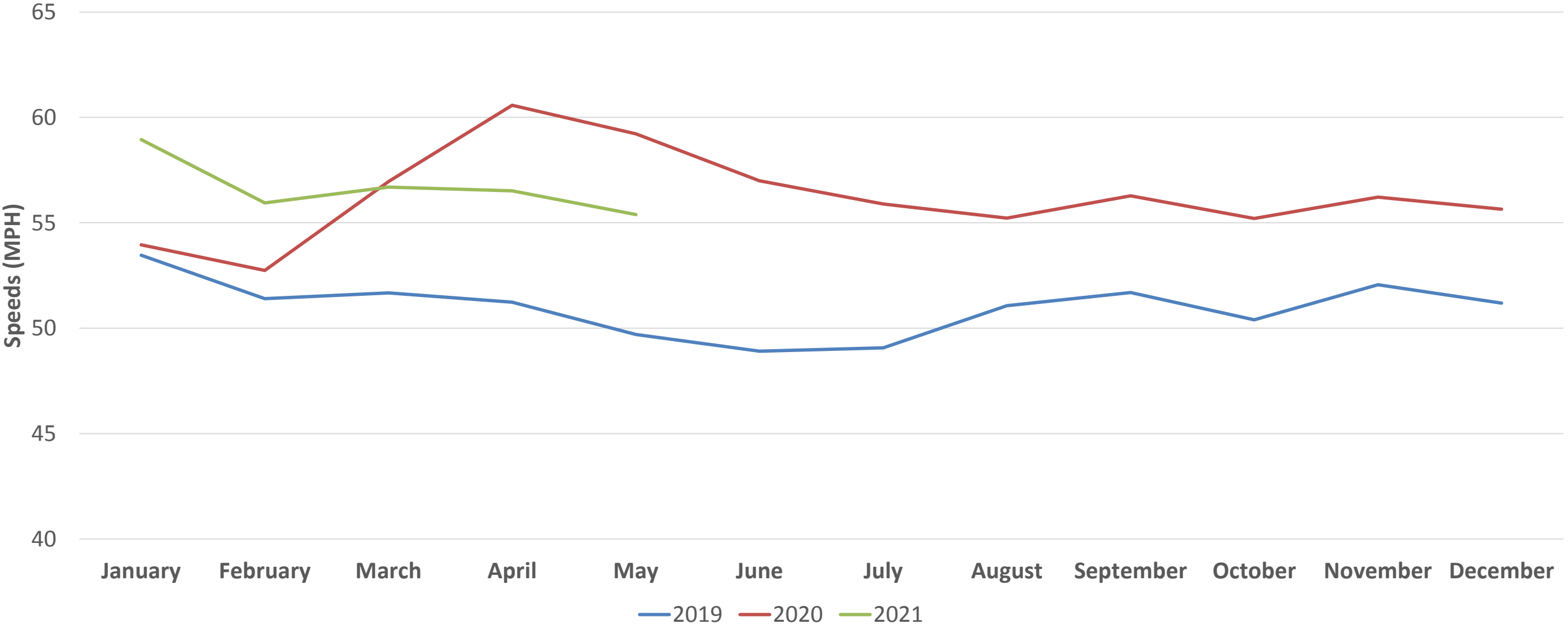
Weekday Truck Speeds on Interstate Highways
